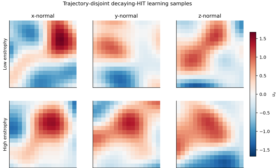
Figure 4: Orthogonal streamwise-velocity slices from representative low- and high-entrophy learning crops. Both rows use one common physical colour scale; the group names denote local vorticity strata, not geometric position.
